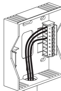
Surface-mounted connection
