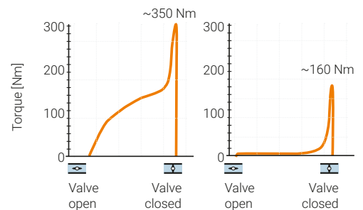
Conventional butterfly valve DN 300
