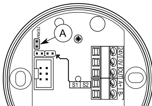
A. TERM jumper
